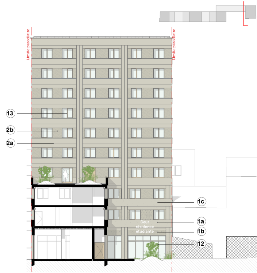
FACADE OUEST _ COUR RESIDENCE ETUDIANTE
